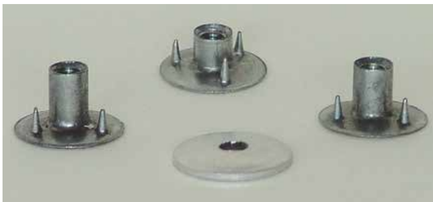
Art. 302 Base filettata in alluminio - conf. 50 pz. per misura Threaded aluminium bases mm. 7, 8, 10, 12 - 50 piece pack
